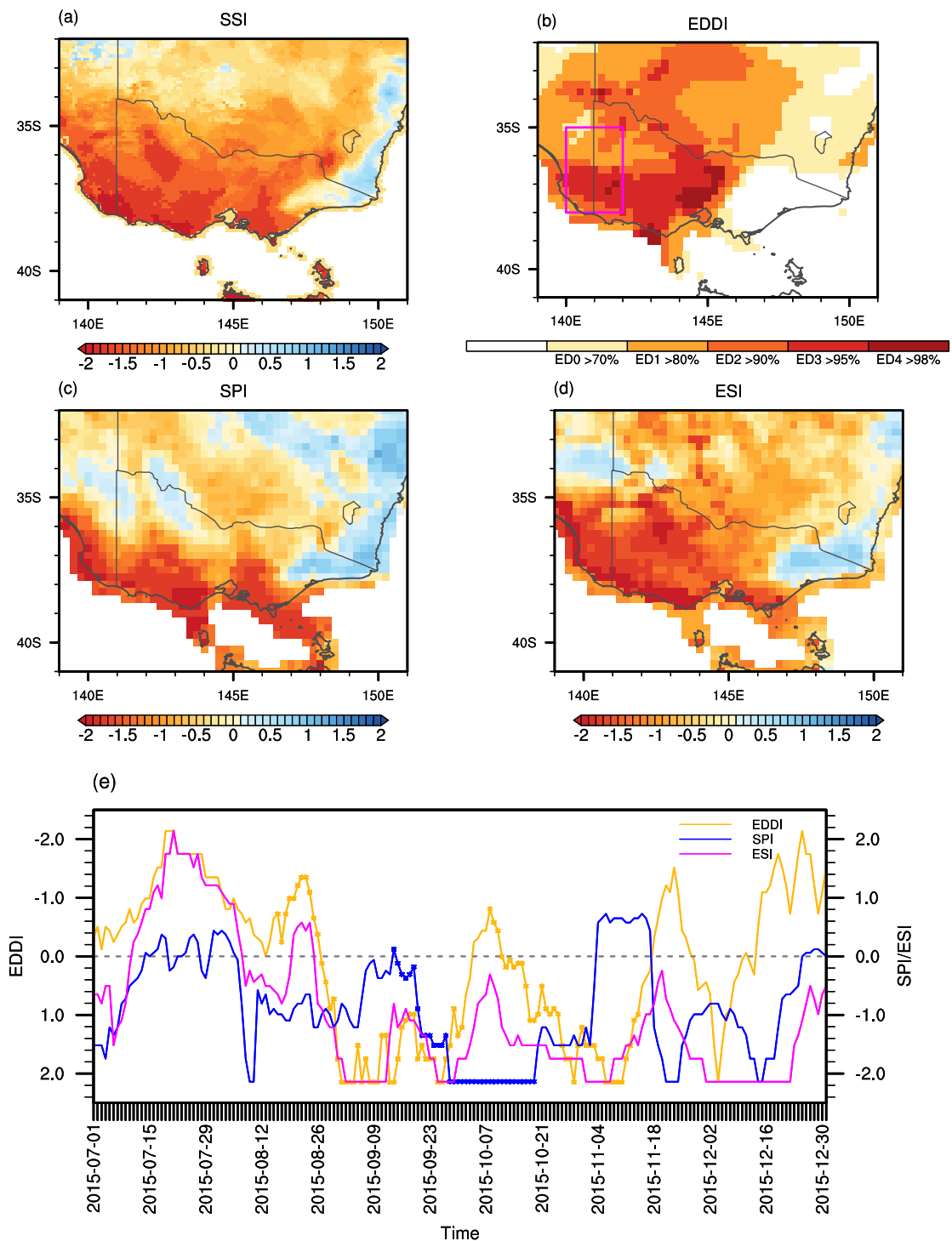
Figure 5. For 28 October 2015: (a) SSI index; (b) EDDI categories for pixels at which the definition of a flash drought using EDDI values is satisfied (the drought categories and percentiles are given in the colour bar—percentiles of between 30% and 70% indicate no effect, and below 30% are wetness categories); (c) SPI index; and (d) ESI index, as per the colour bars. The Wimmera region is approximated by the magenta rectangle in (b). (e) Time series for the period 1 July to 31 December 2015 for an example location at 37°S, 140.5°E for: EDDI (orange line, left vertical axis), and SPI (blue line) and ESI (magenta line, both right vertical axis). Note the reversal of the scale on the left vertical axis, as positive EDDI values correspond to drought, which is indicated by negative values of the other indices. Flash droughts as defined for each index are indicated by asterisks.
